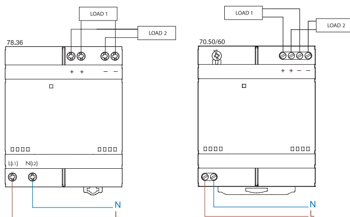
Raccordement double
