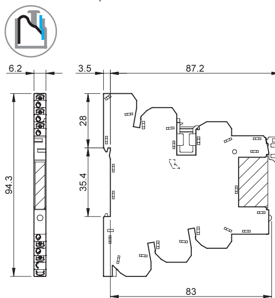
Types 39.60/39.60.3 39.61/39.61.3 Bornes automatiques
