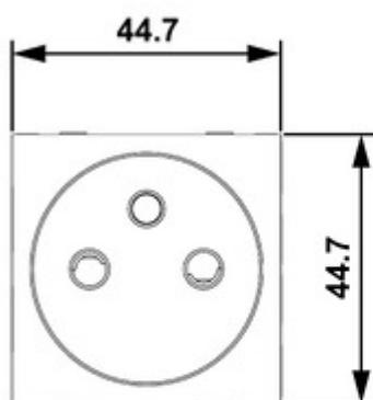
Dimensions (mm)
