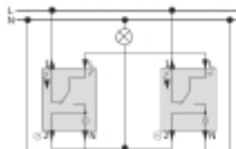
Two-way switch with indicator light Mux3106-0000
