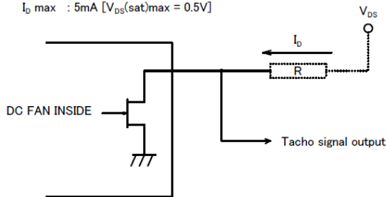
TACHO SIGNAL CIRCUIT
